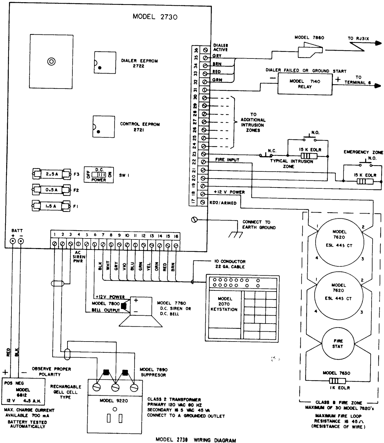
MODEL 2730 WIRING DIAGRAM
