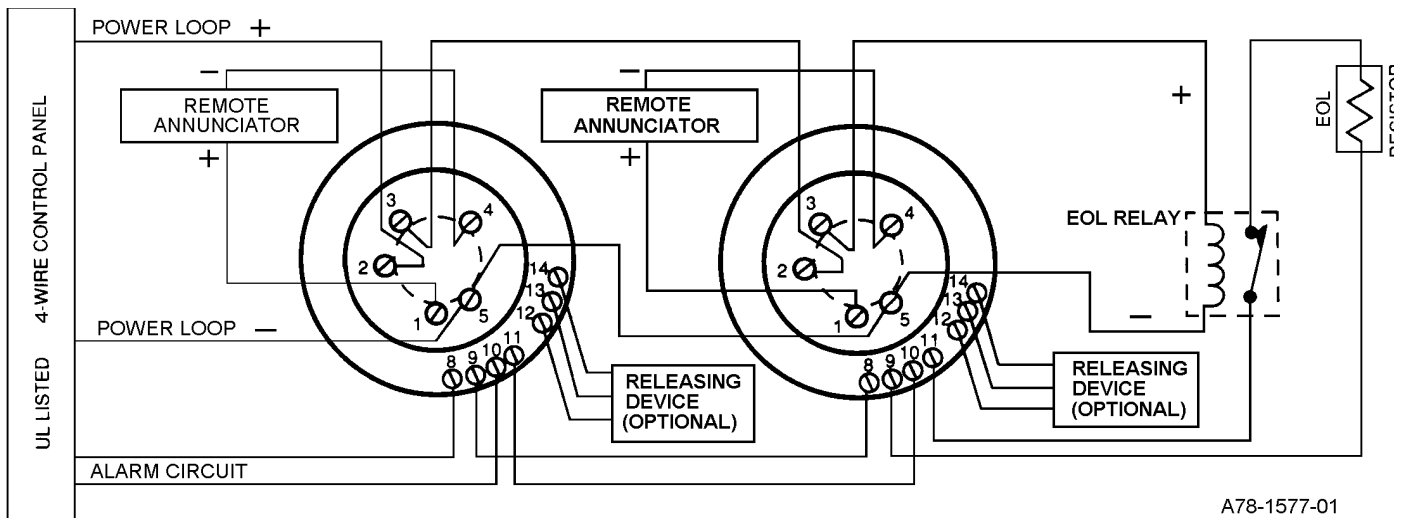
Figure 2. Typical Wiring Diagram
