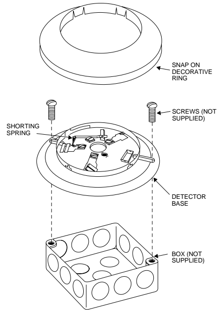
Figure1. Mounting Base to Box
