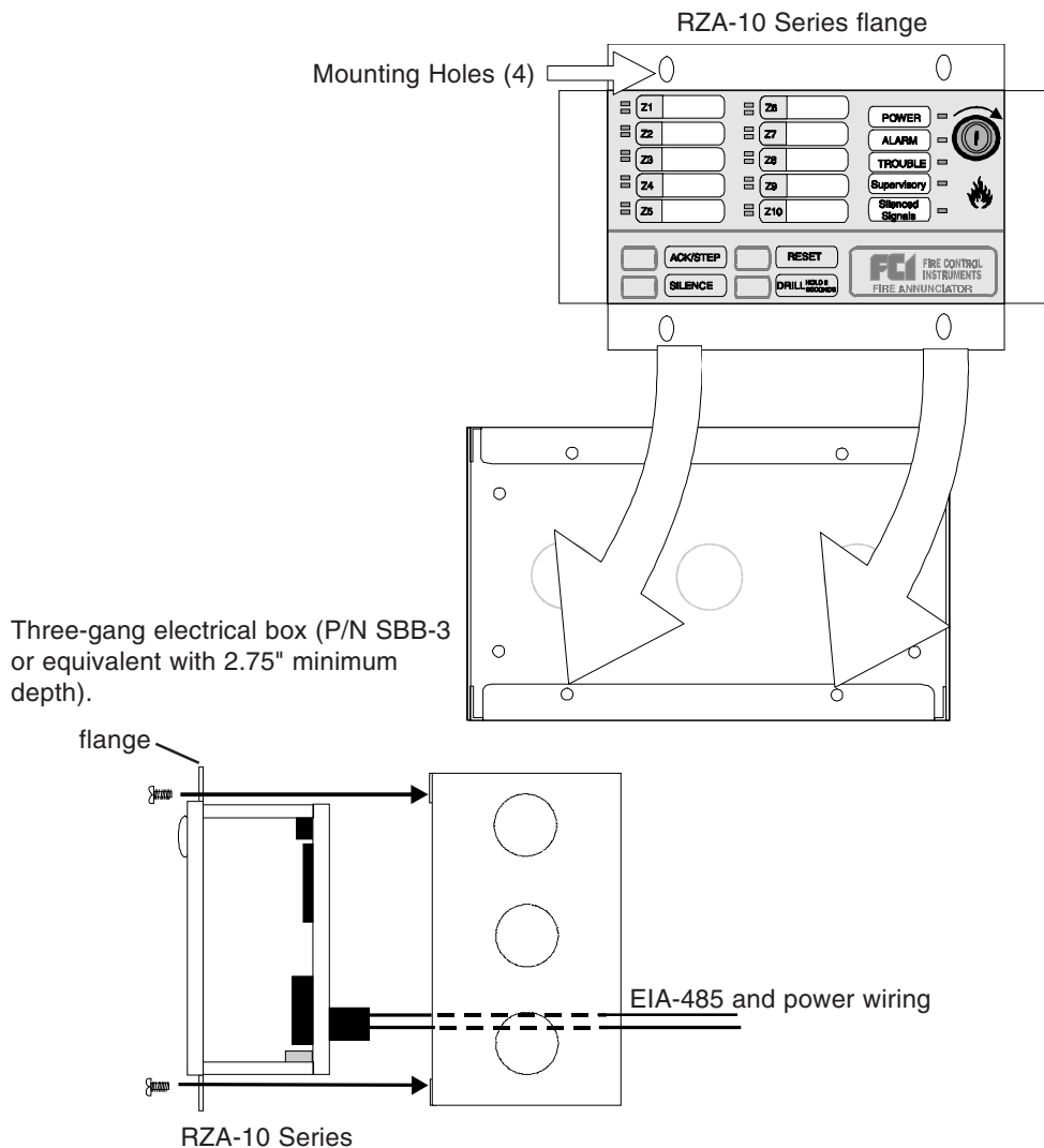
Figure 2-4: Surface Mounting
