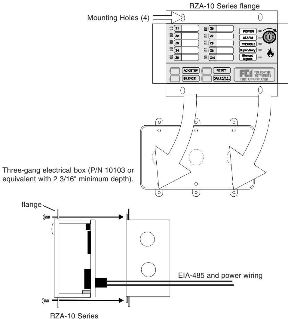
Figure 2-3: Semi-flush Mounting
