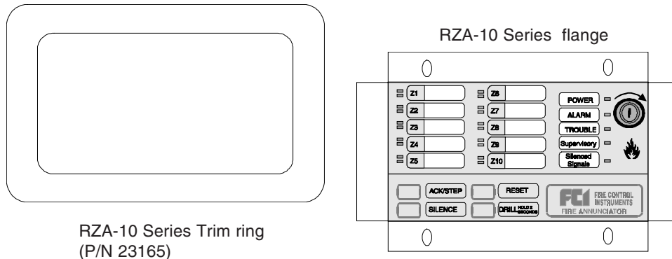
Figure 2-1: RZA-10 Series Hardware
