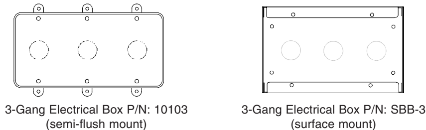
Figure 2-2: RZA-10 Series Backboxes
