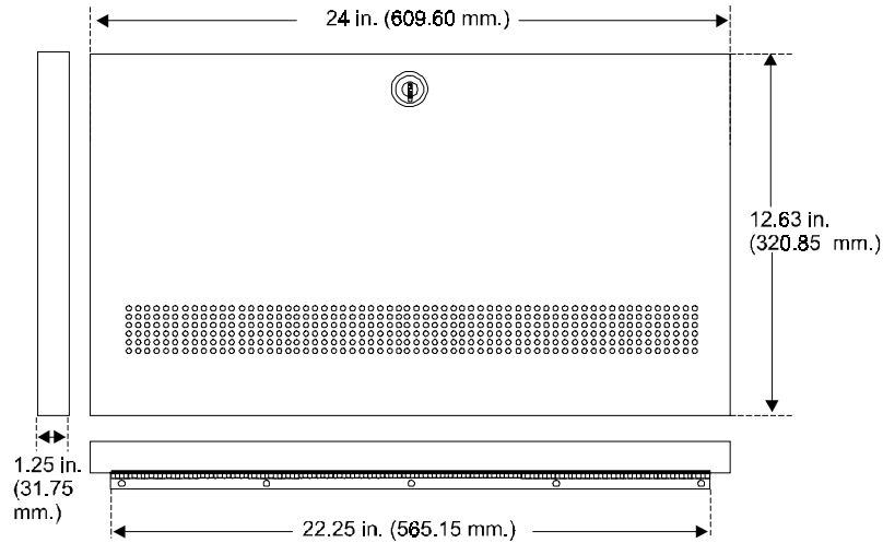
Cabinet Door, hinged at bottom
