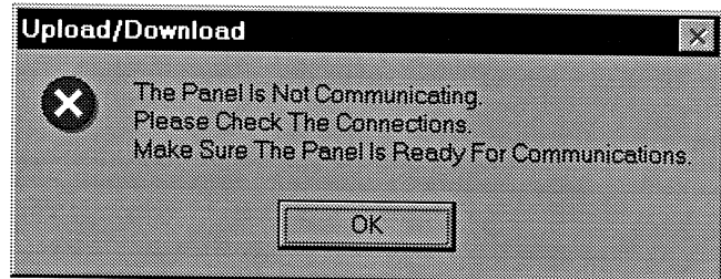
Figure 10-5: Communication Fault
