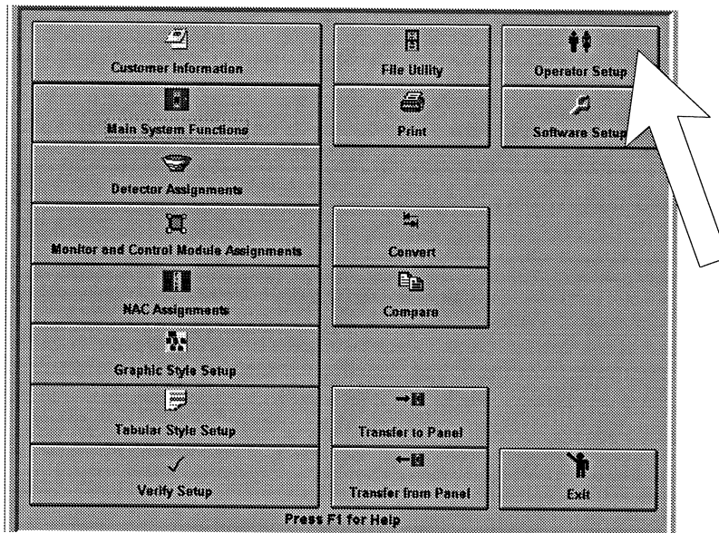
Figure 3-5: Main Menu
