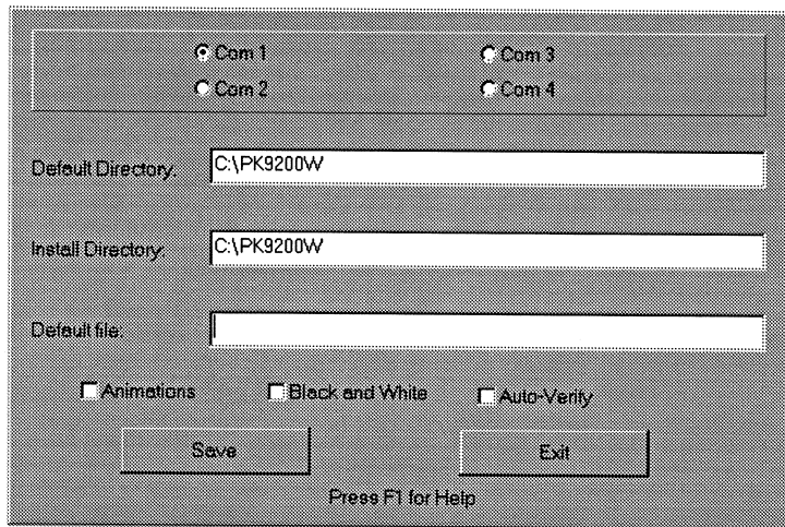
Figure 3-8: Software Setup
