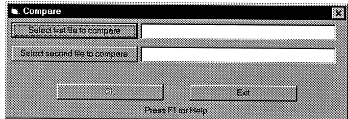
Figure 9-1: Compare Screen
