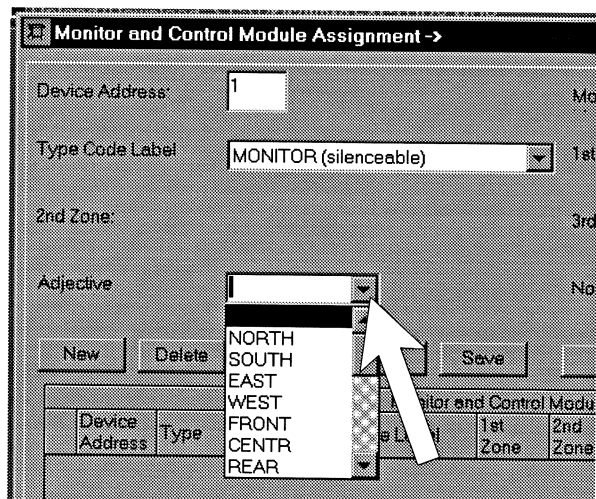
Figure 3-33: Adjective
