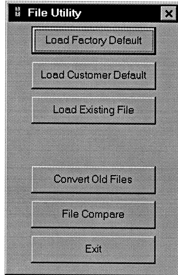
Figure 7-1: Load File
