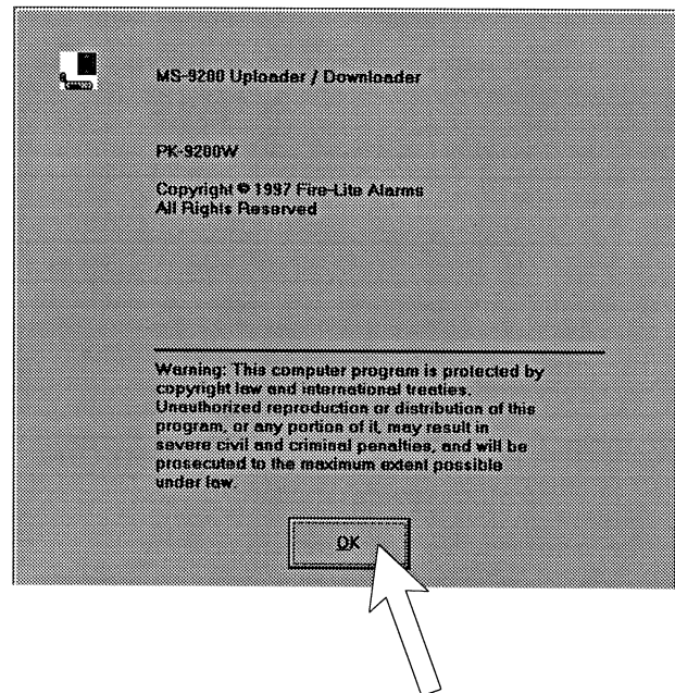
Figure 3-2: Copyright Screen
