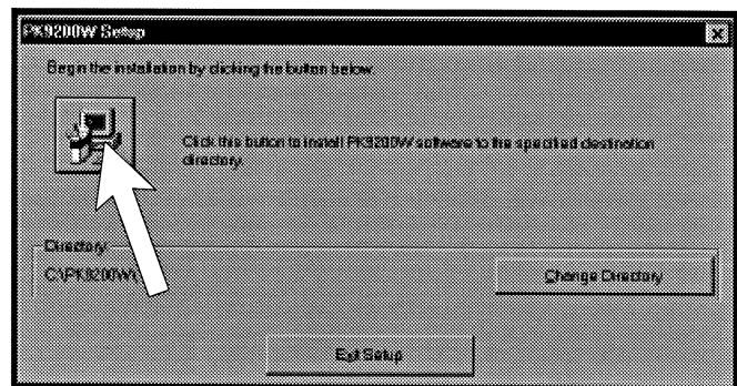
Figure 2-5: Installation Path
