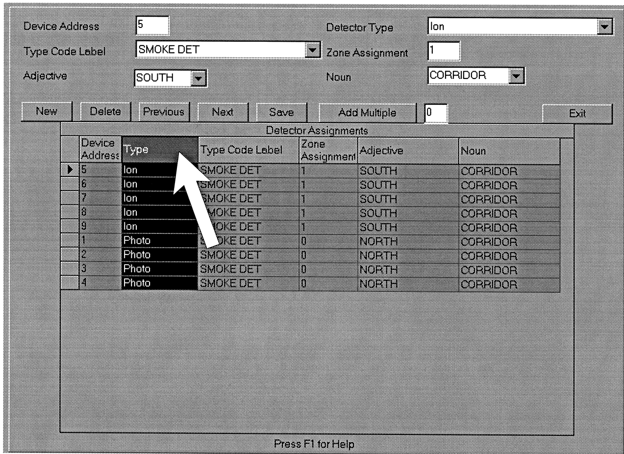
Figure 3-28: Sorting Detectors
