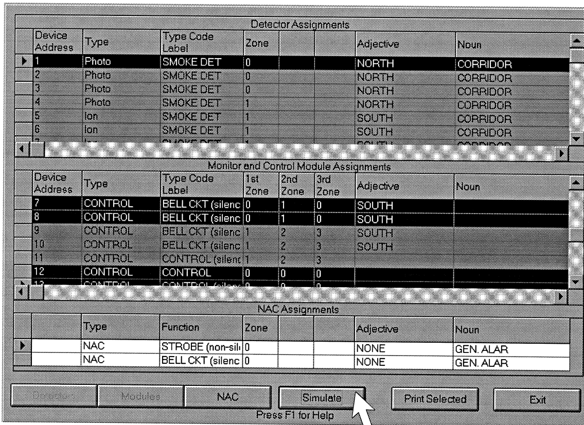
Figure 5-6: Simulate
