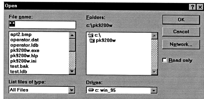
Figure 10-2: File Screen
