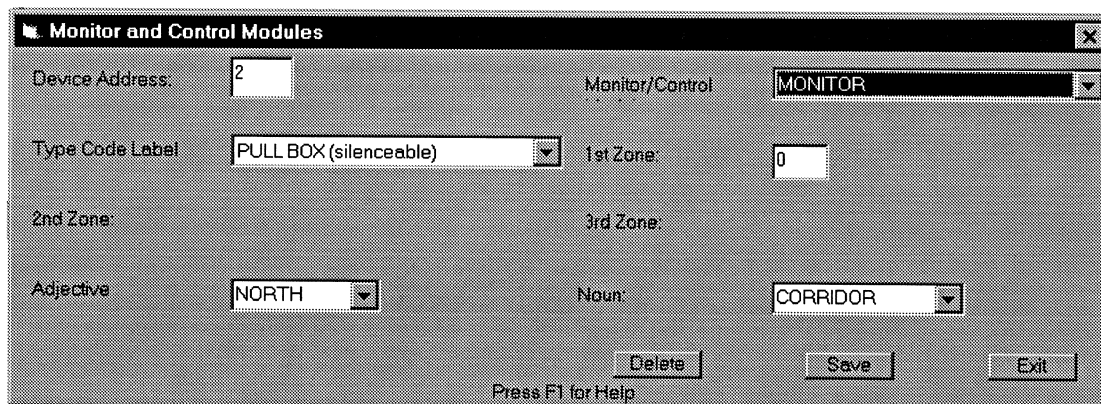
Figure 4-3: Module Editing
