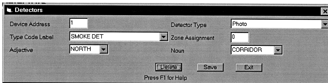
Figure 4-2: Detector Editing
