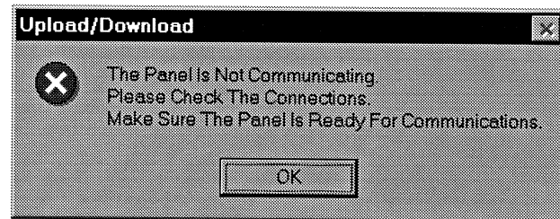
Figure 11-4: Communication Fault
