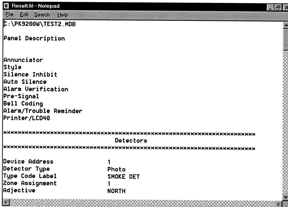
Figure 7-2: Print Notepad
