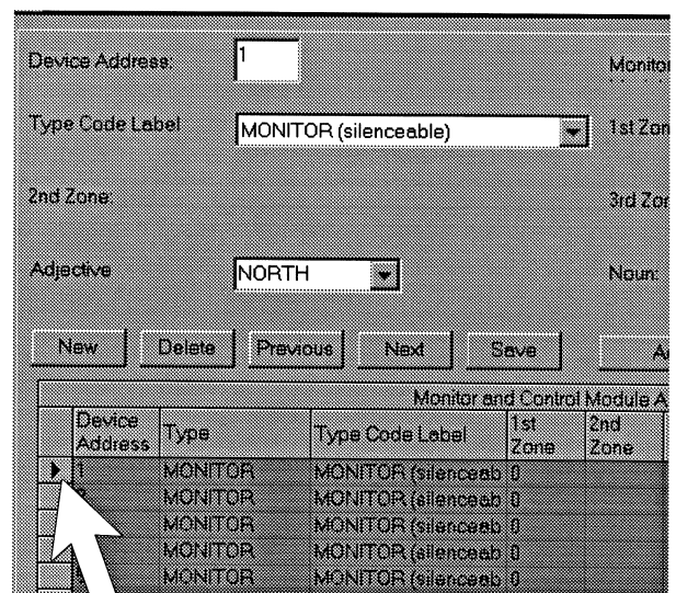
Figure 3-36: Selecting Modules
