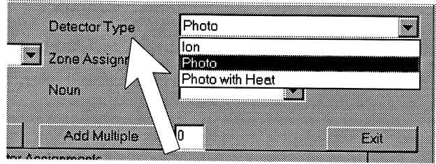
Figure 3-22: Detector Type
