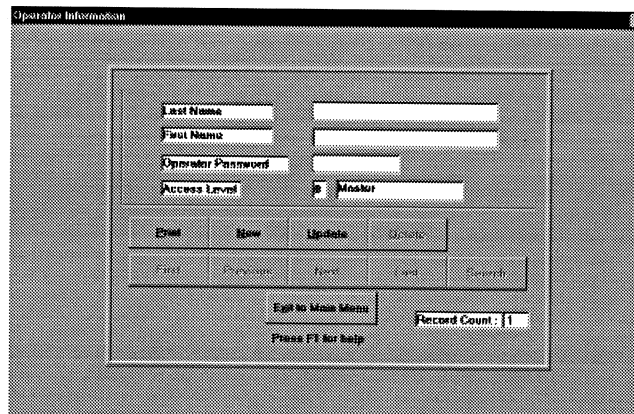
Figure 3-6: Operator Information
