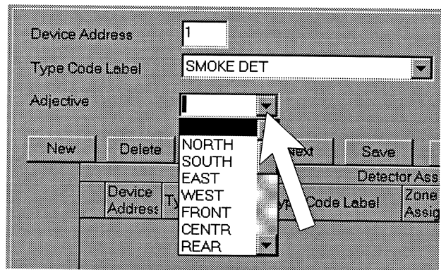
Figure 3-23: Adjective
