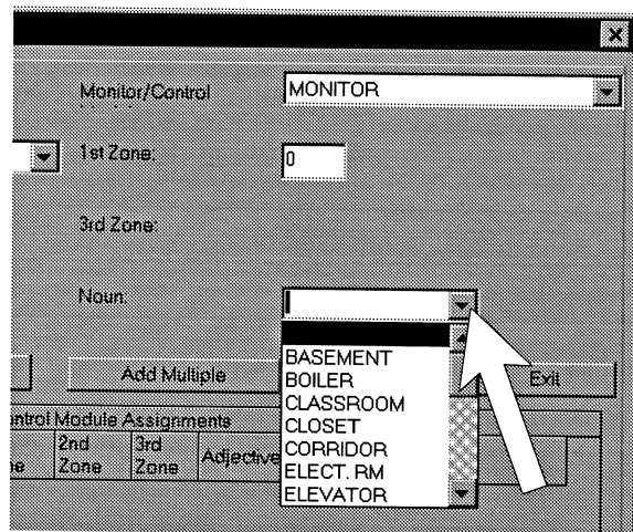
Figure 3-34: Noun
