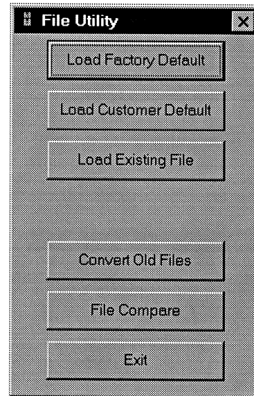
Figure 10-1: Load File
