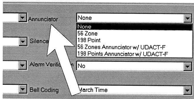
Figure 3-13: Annunciator Options
