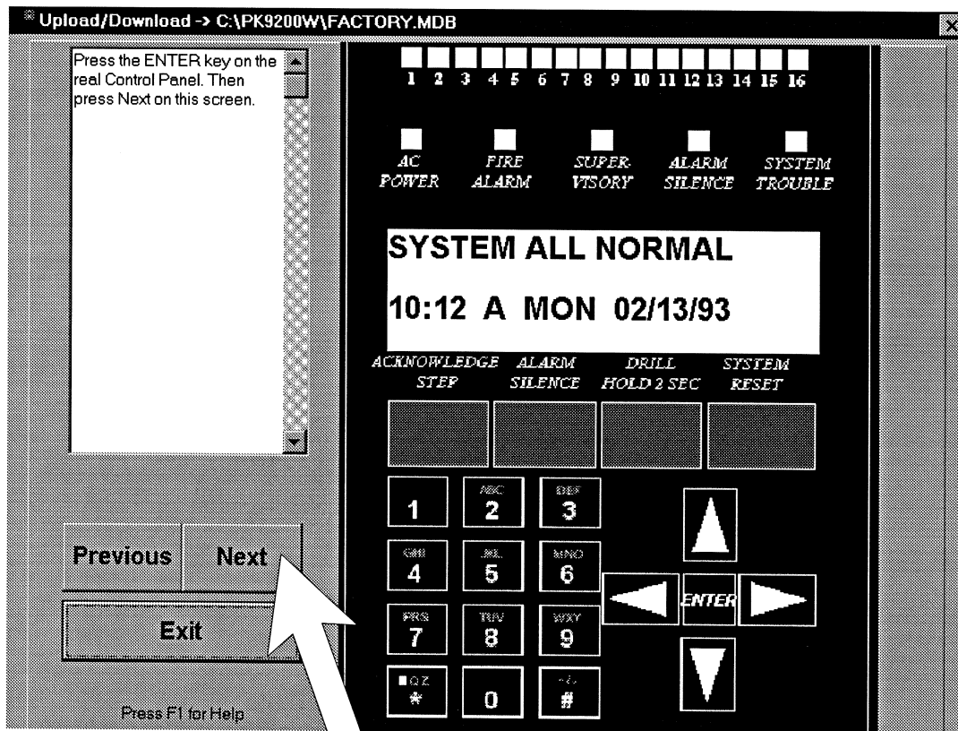
Figure 11-1: Transfer Screen
