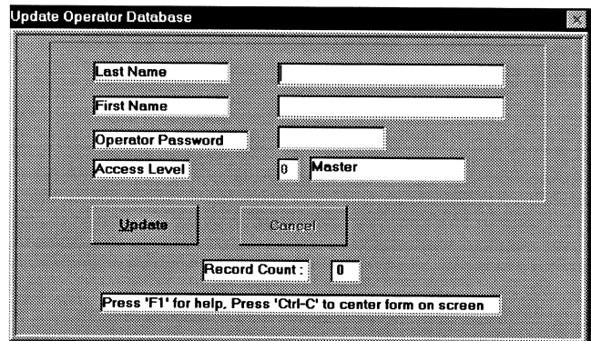
Figure 3-3: Initialization Screen
