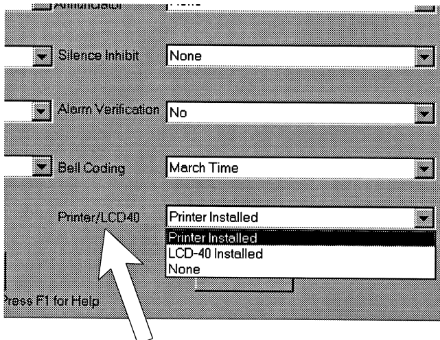
Figure 3-20: Printer/LCD-40
