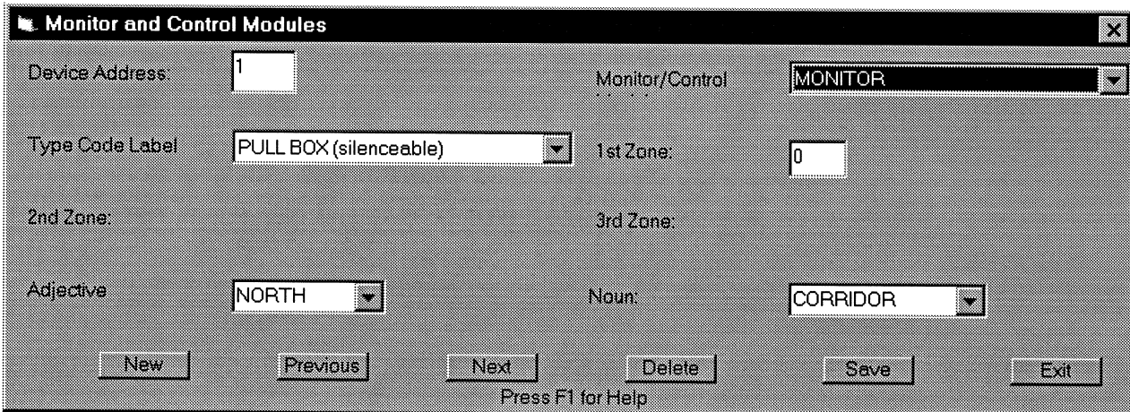
Figure 5-4: Module Setup Screen
