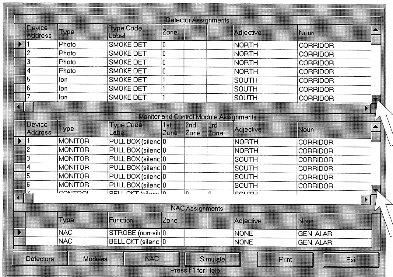
Figure 5-2: Tabular Style Setup Screen
