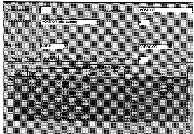
Figure 3-35: Programmed Modules
