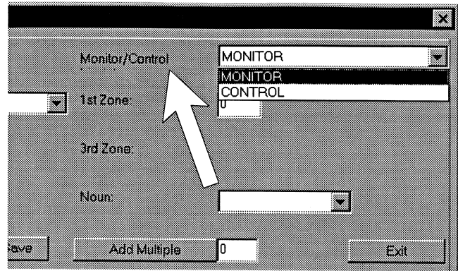
Figure 3-30: Monitor/Control Module
