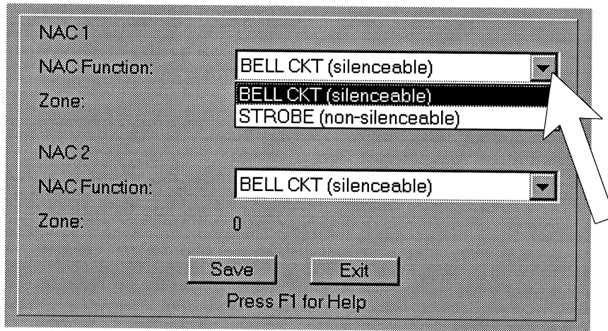
Figure 3-38: NAC Assignments
