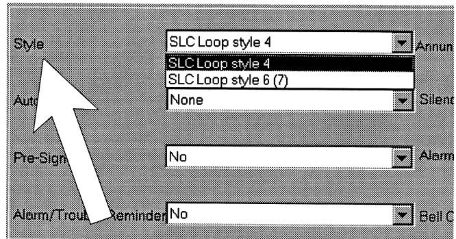
Figure 3-12: Style Options
