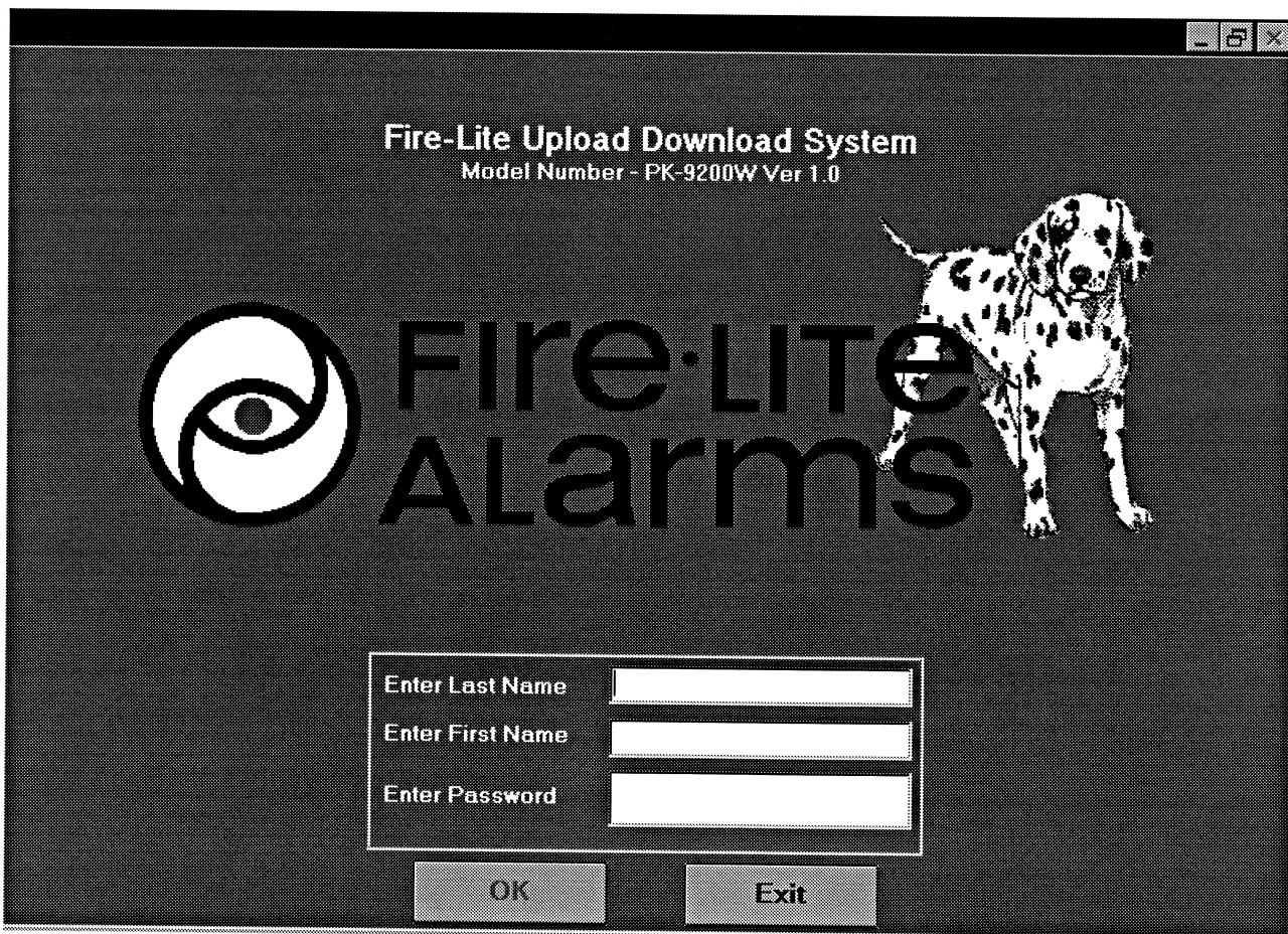
Figure 3-4: Log-in
