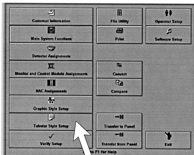
Figure 5-1: Main Menu
