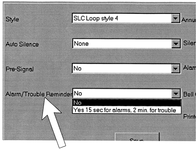
Figure 3-18: Alarm/Trouble Reminder
