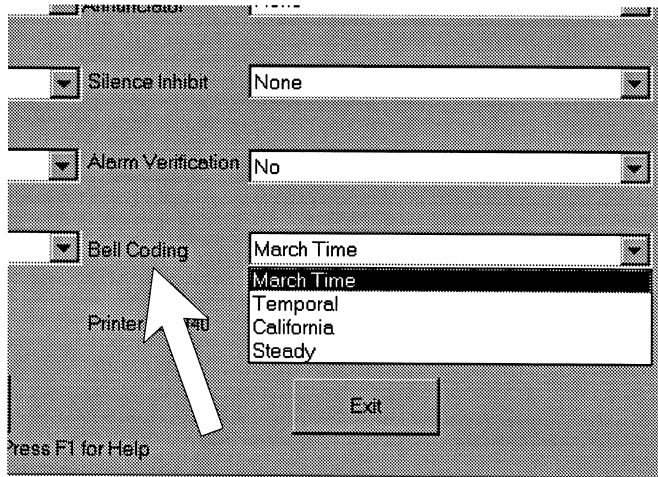
Figure 3-19: Bell Coding
