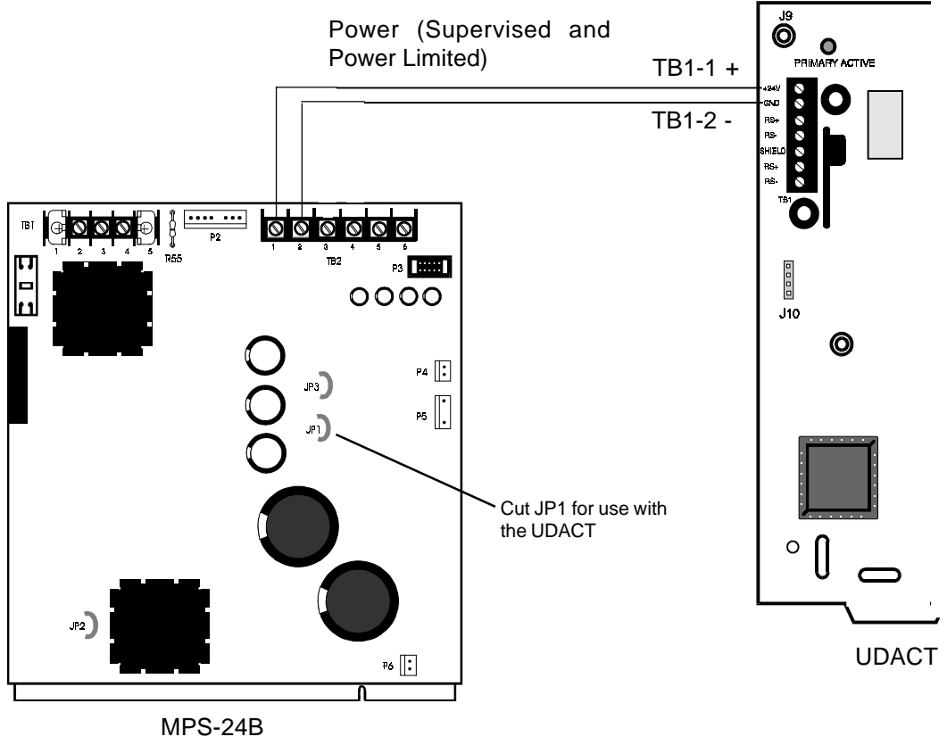
Figure 6-7: 24 VDC Power Connection to UDACT
