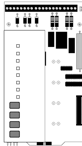
CPU-2000 (Sensican 2000)
