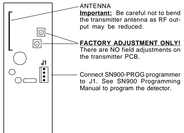
Figure 4 RF Transmitter PCB
