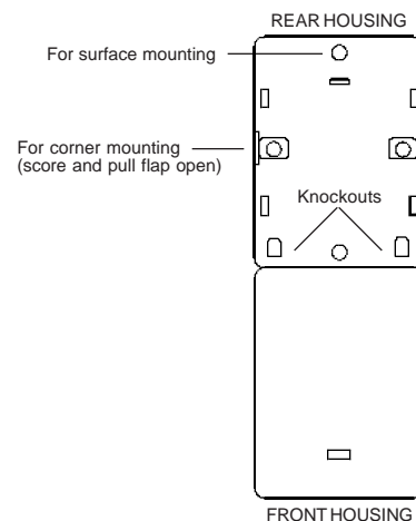
Figure 1 Mounting the FG-715/FG-730
