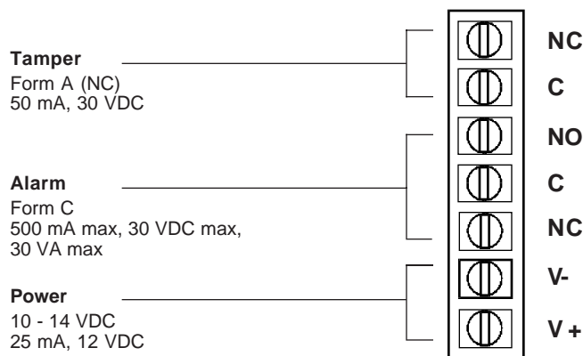
Figure 2 FG-715/FG-730 Terminal Strip
